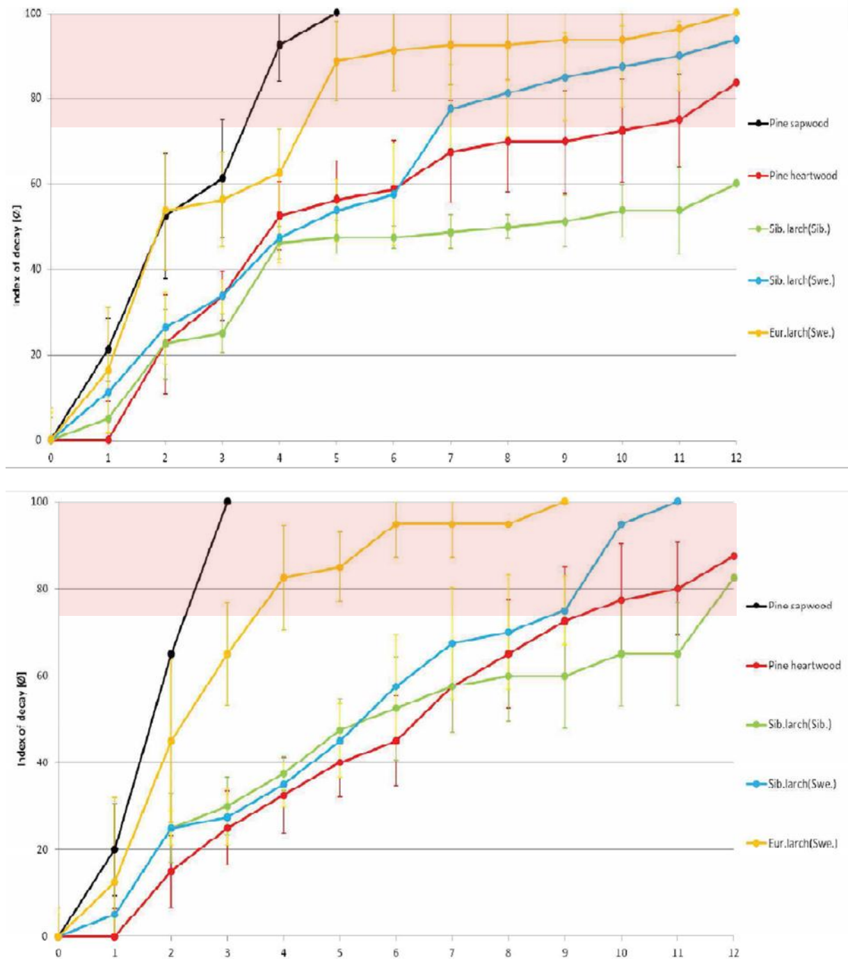
Figure 9 Rot index (or index of decay) for test samples in the ground in accordance with EN 252 from field trials in Simlångsdalen (top) and Ultuna (bottom), where the heartwood (red) and sapwood (black) from pine compared two types of larch ( Larix sibirica , Larix decidua ) from two plant locations Larix sib. from Siberia (green) and from Sweden (blue) and Larix dec. from Sweden (yellow). (Reference: Pockrandt 2012)
